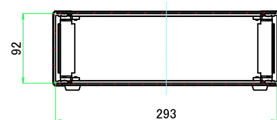
B-B (1:5)
