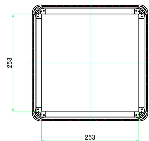
C-C (1:5)
